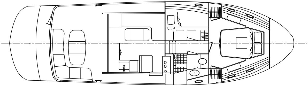
2 cabin floor plan
